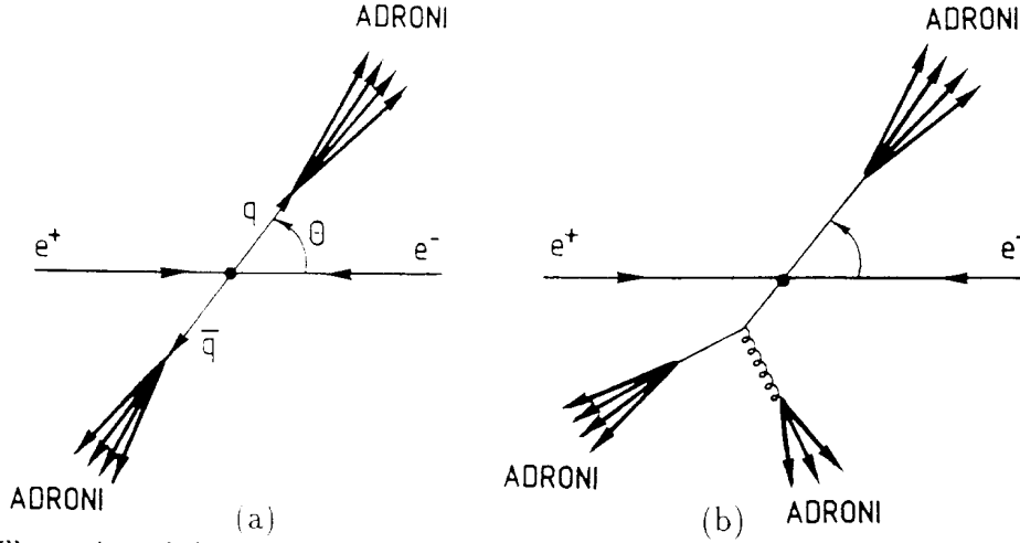
Fig. 3. Illustration of the hadron production processes in e^+e^- collisions. (a) A quark and an antiquark are produced; they then hadronize, leading to a two-jet event. (b) The antiquark emits a gluon; then the quark, the antiquark and the gluon hadronize, leading to a three-jet event.
