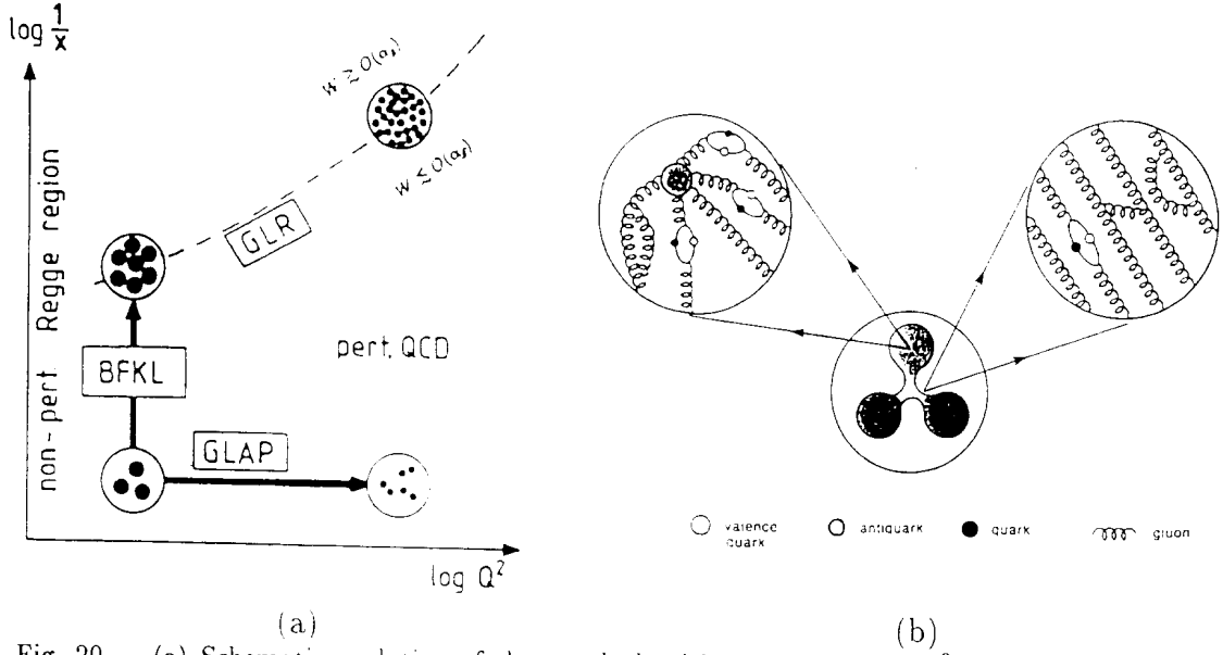
Fig. 20. (a) Schematic evolution of the quark densities in various (x, Q^2) regions according to the main dynamical effects. (b) Schematic nucleon structure. Center: the nucleon made of three constituent quarks interacting via colour force tubes. Left: a close up reveals the sea of virtual particles around the valence quarks. Right: a close up of a colour tube reveals the gluons that carry the colour force, and which can fluctuate into q\bar{q} pairs.
