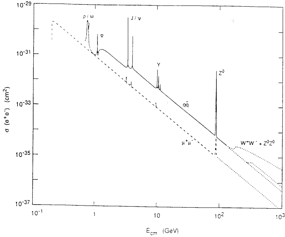
Fig. 1. Energy dependence of \sigma(e^+e^- \rightarrow \text{hadrons}) and \sigma(e^+e^- \rightarrow \mu^+\mu^-) .
