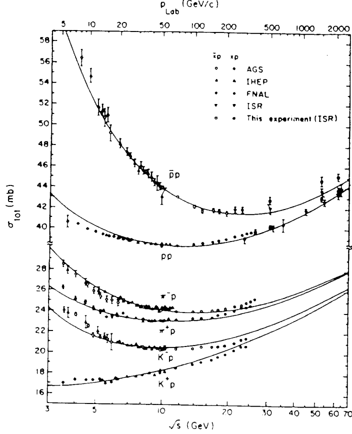
Fig. 11. Total cross-sections for high-energy hadron-hadron scattering. The curves are computed according to Lipkin's parametrization.
