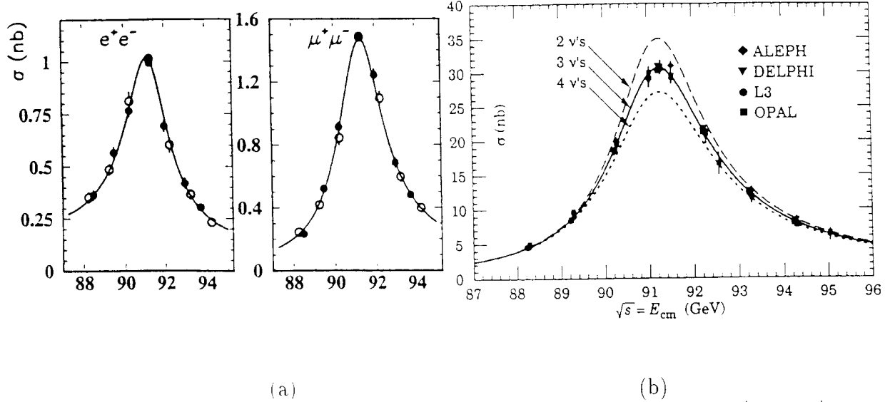
Fig. 4. (a) The measured cross-sections for e^+e^- \rightarrow e^+e^- (for |\cos\theta| < 0.7 ) and e^+e^- \rightarrow \mu^+\mu^- . The lines are the results of the fits to all the data. (b) Measured hadron data compared with the predictions of the Standard Model for two, three and four generations 2 .
