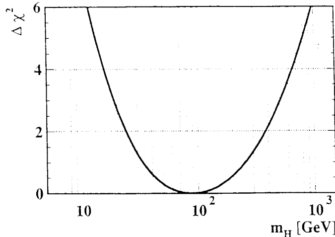
Fig. 5. The \Delta\chi^2 for the fit of the electroweak precision measurements versus m_H 1 .
