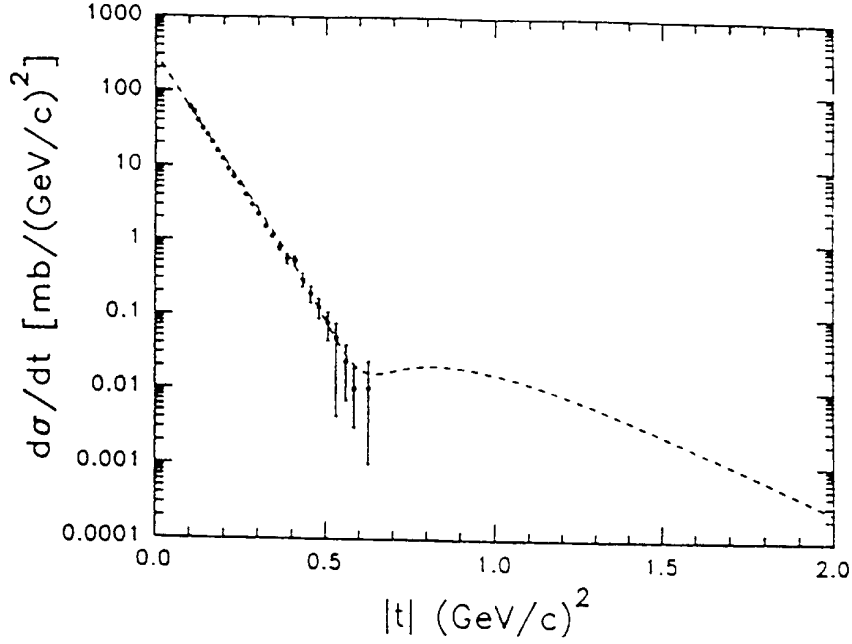
Fig. 14. Differential elastic scattering cross-section for \bar{p}p at \sqrt{s} = 1.8 GeV at Fermilab together with a fit by Block et al. 8 .
