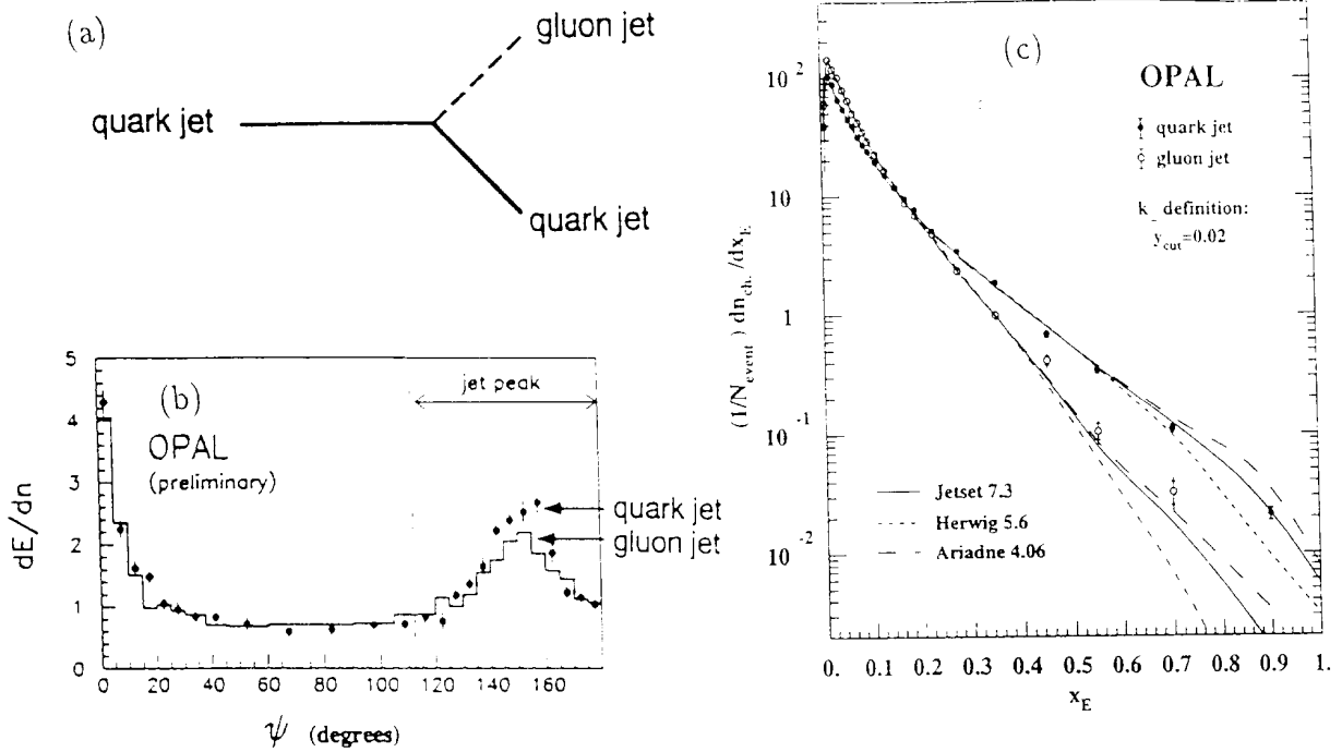
Fig. 9. (a) The chosen symmetric topology to study quark gluon jet differences; (b) the angular distribution of jet energy and (c) the charged particle fragmentation functions.
