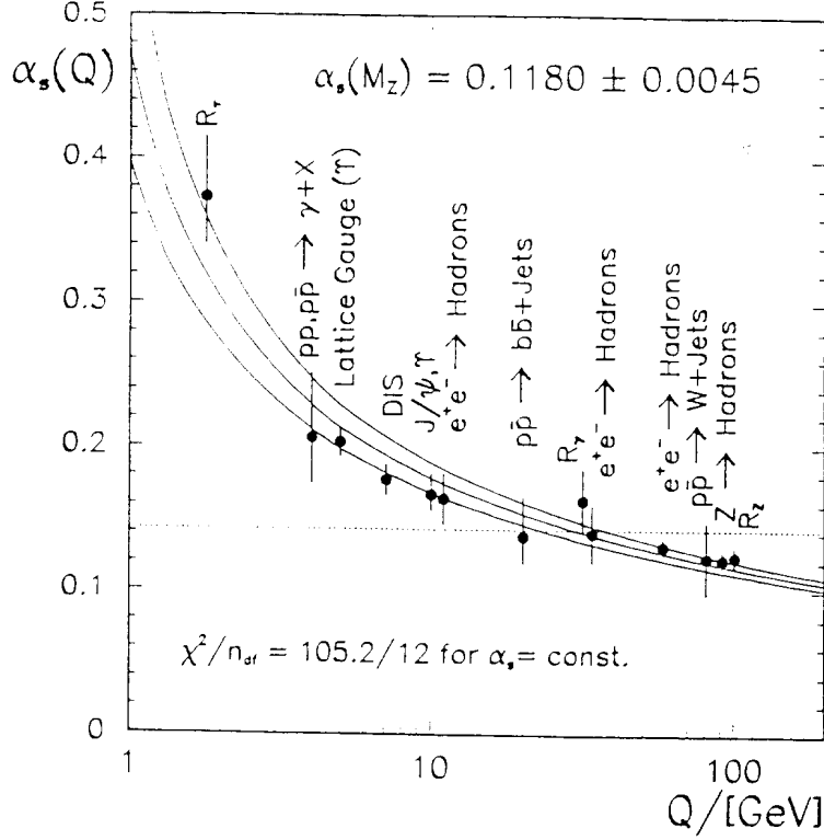
Fig. 8. A summary of measurements of \alpha_s , compared with QCD expectations for \alpha_s(m_Z) = 0.1180 \pm 0.0045 and N_f = 5 flavours.
