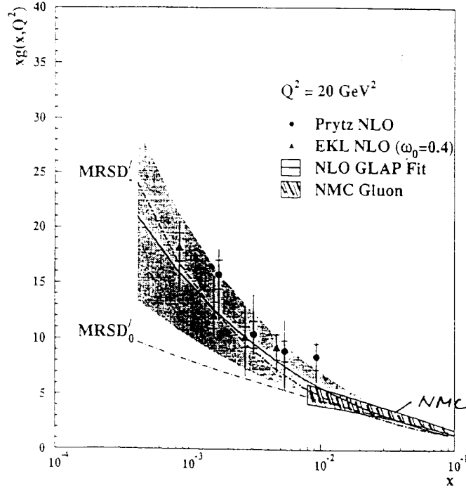
Fig. 19. The gluon structure function from the ZEUS and the NMC experiments for x < 0.1 .
