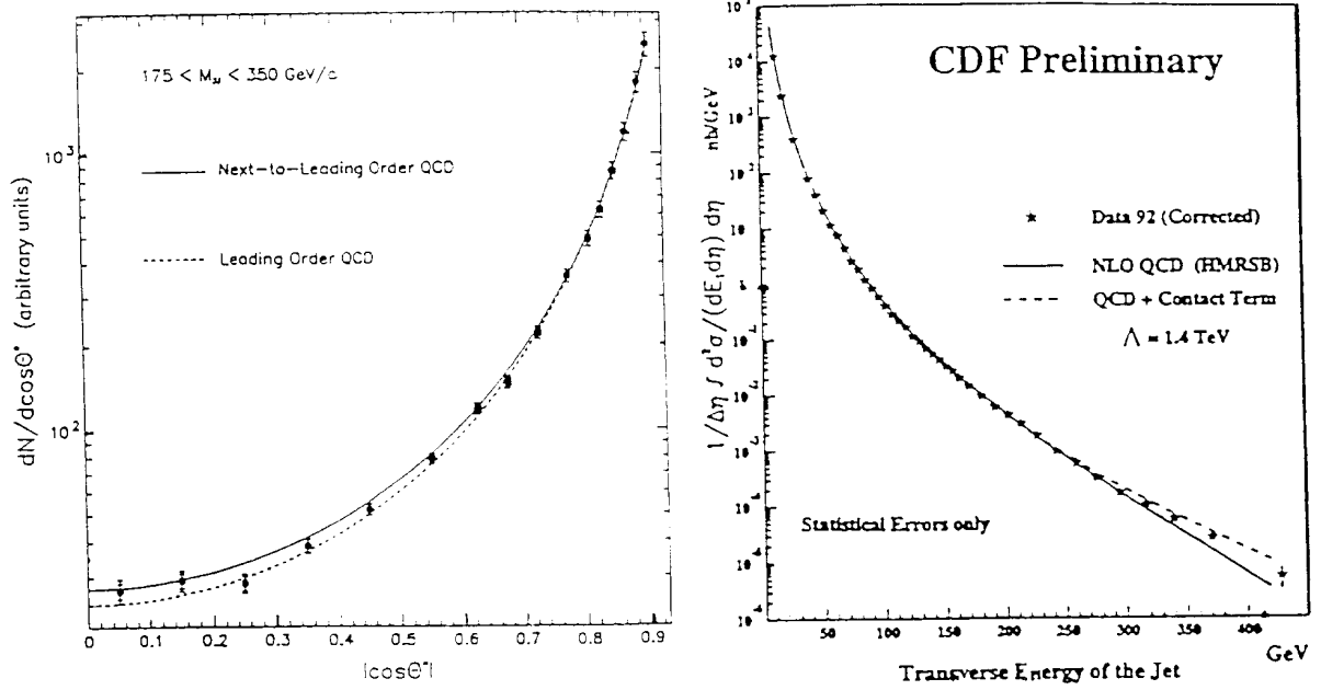
Fig. 15. (a) Inclusive jet cross-section referred to the p\bar{p} line of flight; (b) angular distribution of parton-parton scattering 10 .
