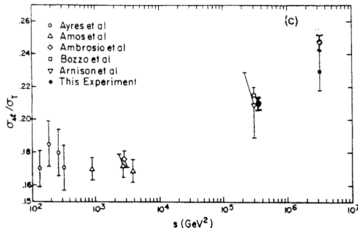
Fig. 13. Ratio of the elastic to total cross-section for \bar{p}p versus s .
