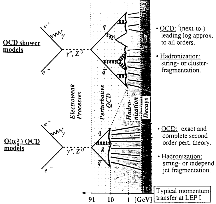
Fig. 6. Model of multihadronic production in e^+e^- collisions.
