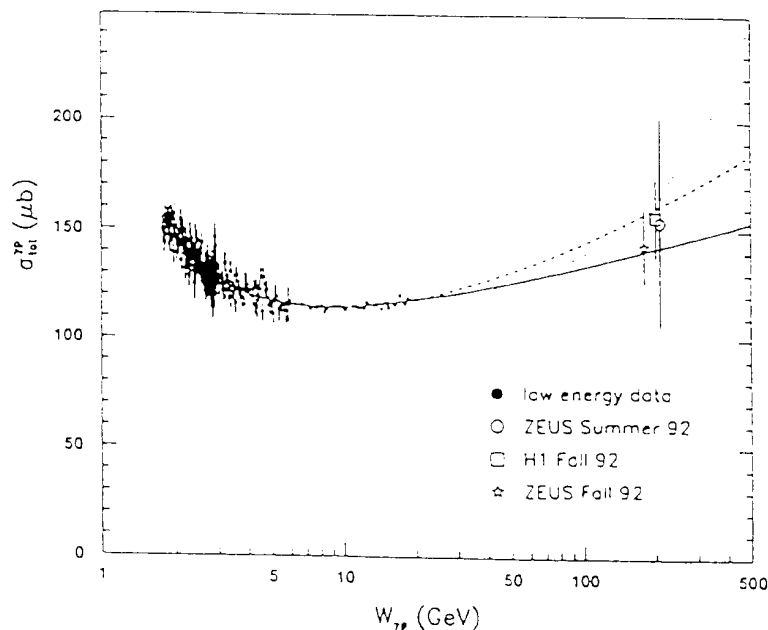
Fig. 21. Total \gamma p cross-section versus c.m. energy, including the “indirect measurements” at HERA.
