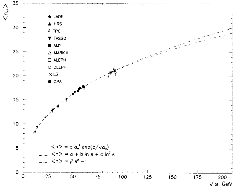
Fig. 7. Average charged multiplicity in e^+e^- collisions plotted versus c.m. energy.
