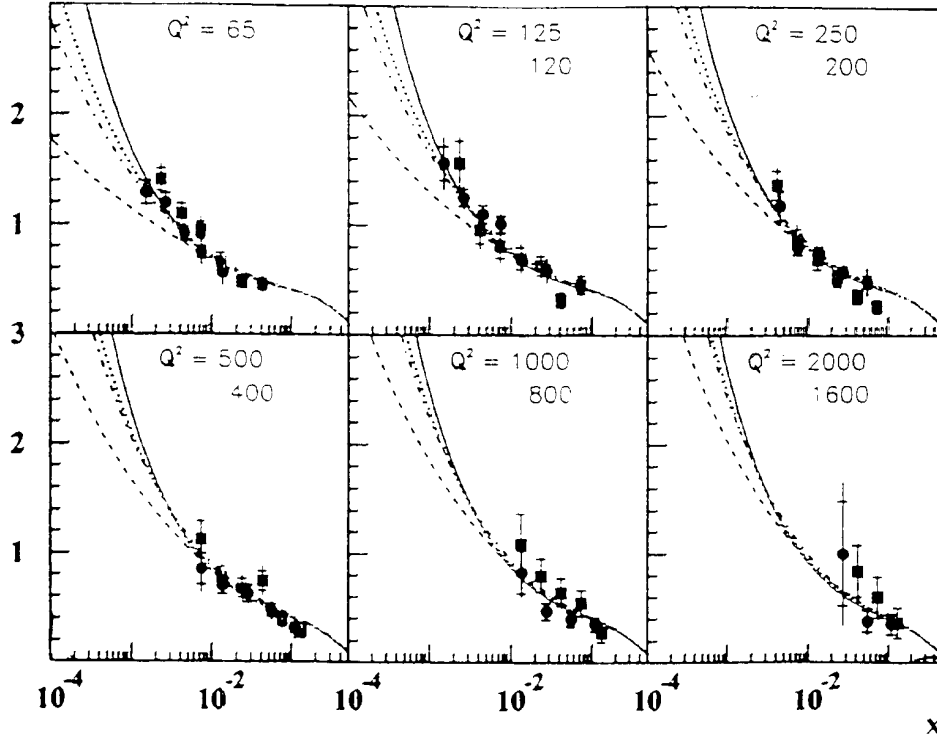
Fig. 18. The proton structure function F_2 from H1 and ZEUS versus x_B for various values of Q^2 .
