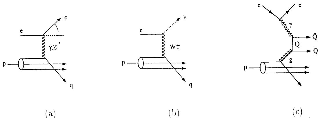
Fig. 16. The basic processes contributing to deep-inelastic scattering: (a) neutral current scattering, (b) charged current scattering and (c) photon-gluon fusion.
