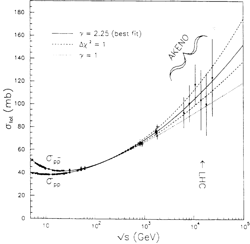
Fig. 12. Compilation of pp and p\bar{p} total cross-sections including cosmic ray measurements. The solid line is a fit of the \sigma_{\text{tot}} and \rho data with dispersion relations 5-8 ; the region of uncertainty is delimited by dashed lines.
